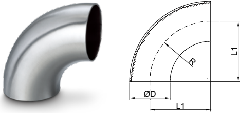
90°焊接式弯头 90° Welded Elbow
