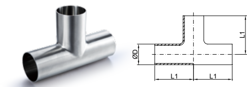
焊接式三通 Welded Tee
